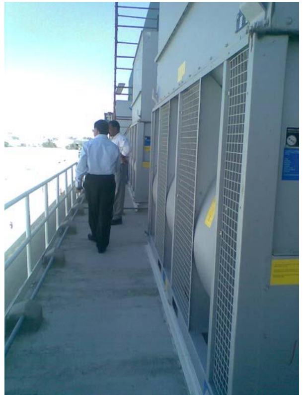
Figure 6- Evaporative Condensers
